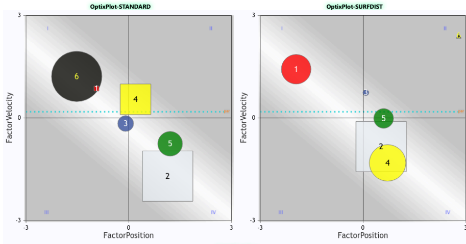
Past 3 Runlines
